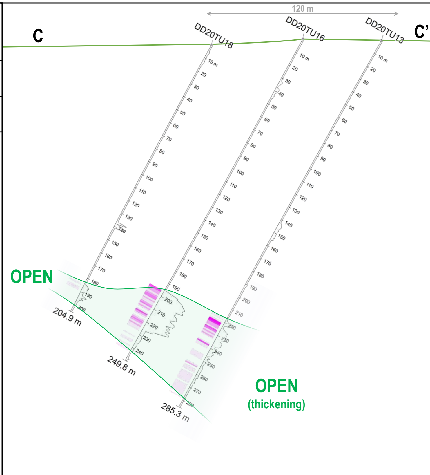
Figure 7: Cross Section of DD20TU16, with Up-Dip Hole DD20TU18 and Down-Dip Hole DD20TU13
