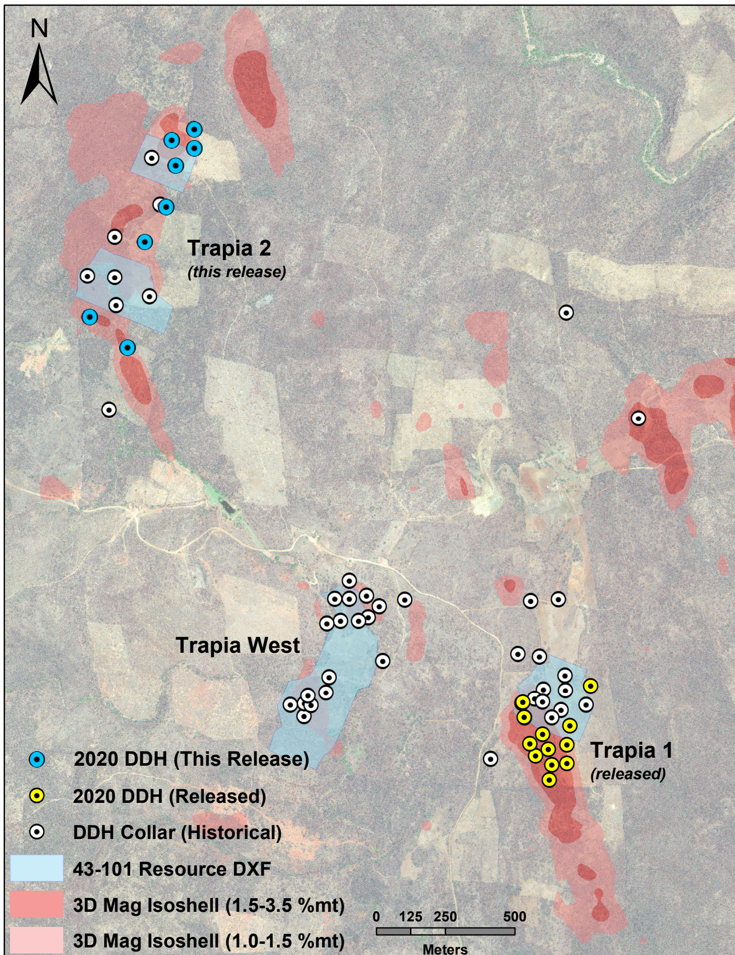
Figure 2: Location of 2020 Drill Holes at Trapia 1 and Trapia 2, and Prospective 3D Magnetic Inversion Drill Targets
